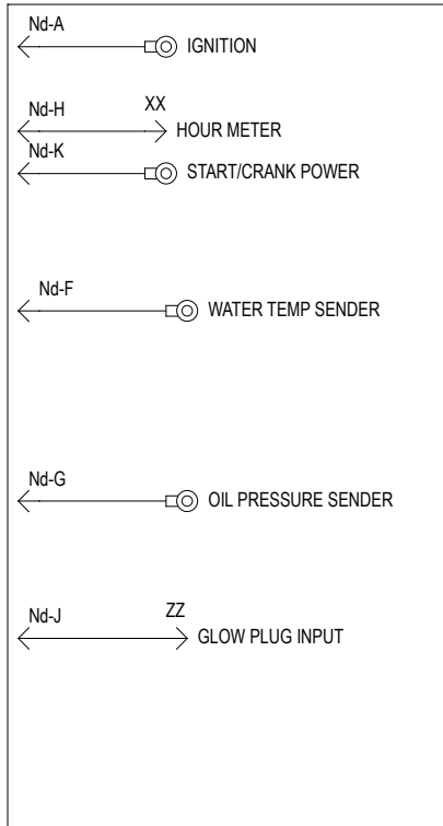
ENGINE SYSTEM S4Q2 DIESEL 0895-136
