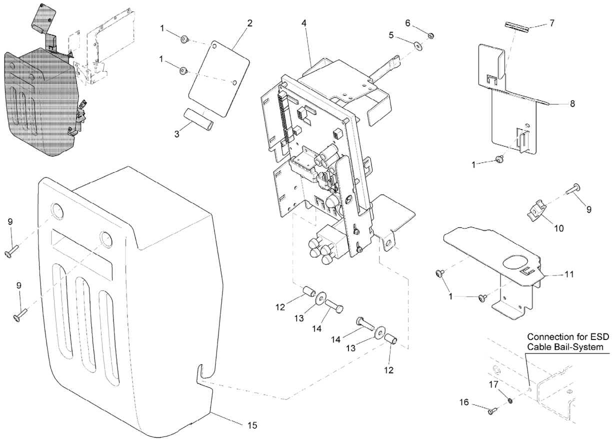
Control Box Electrical Part I (Ref. 97098990-1)
