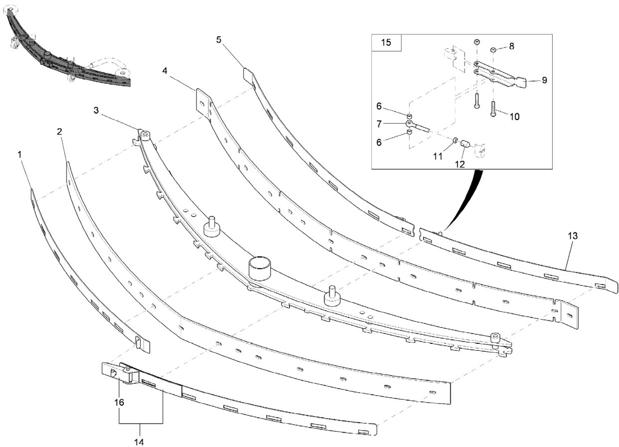
Squeegee Assembly Part I (Ref. 97094502-1)
