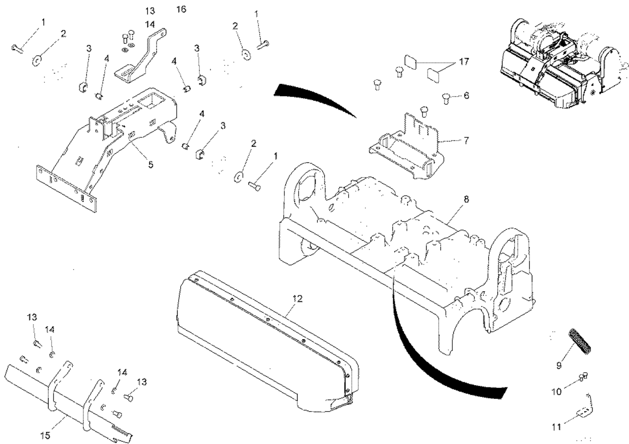
Scrub Deck Assembly Cylindrical (Ref. 97099444-1)
