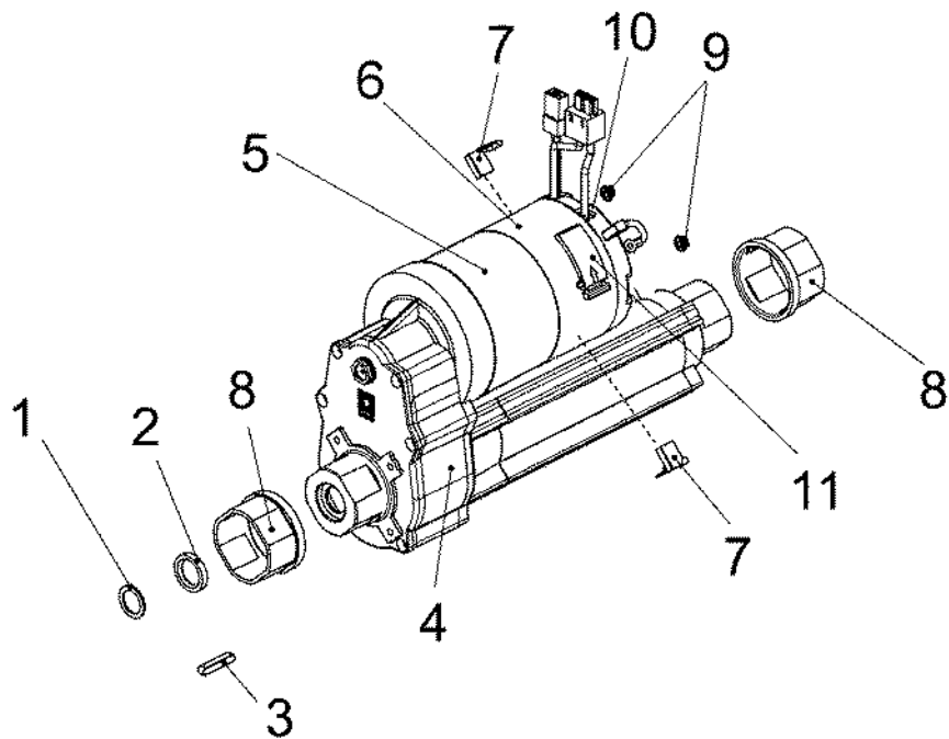
Traction Drive (Ref. 90531609)
