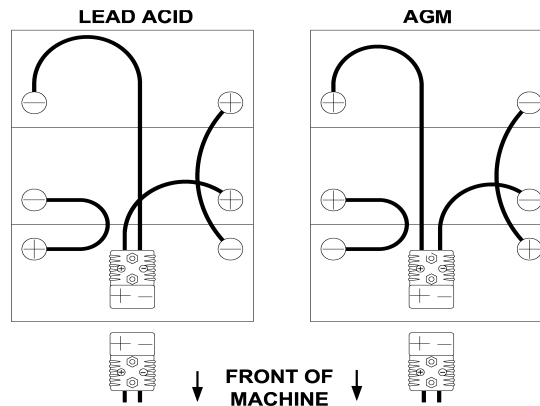
Battery cable routing (Fig. 1/2)
